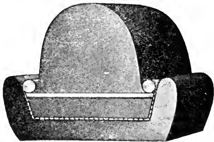
GOODRICH SIDE-WIRE TIRE.
